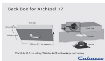
Back Box Archipel 13 & 17
